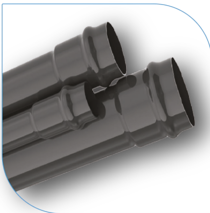
Pipe With O-Ring Gasket Socketed PN 4, PN 6, PN 10, PN 16 Ø 20 - 500
